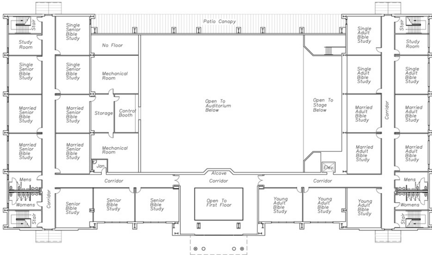
01 SECOND FLOOR PLAN SCALE 3/32" = 1'-0" NORTH
